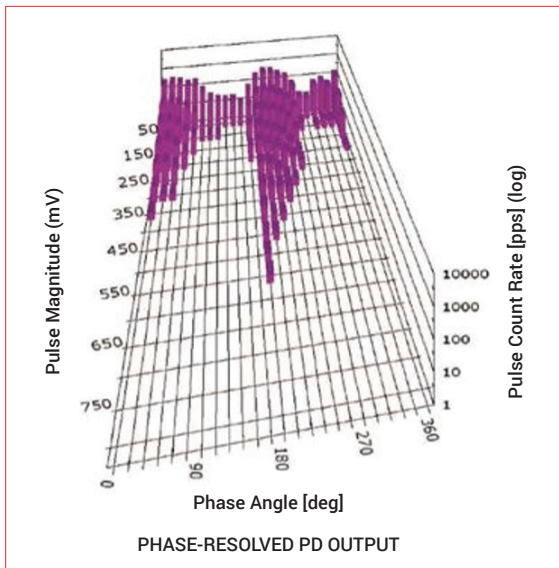
ELECTRICAL TRACKING OF HIGH VOLTAGE BUS DUE TO CONTAMINATION
